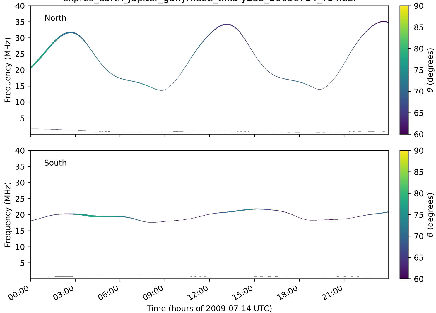
expres_earth_jupiter_ganymede_txka-y235_20090714_v14.cdf
