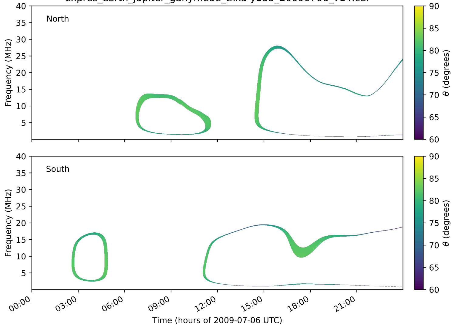
expres_earth_jupiter_ganymede_txka-y235_20090706_v14.cdf
