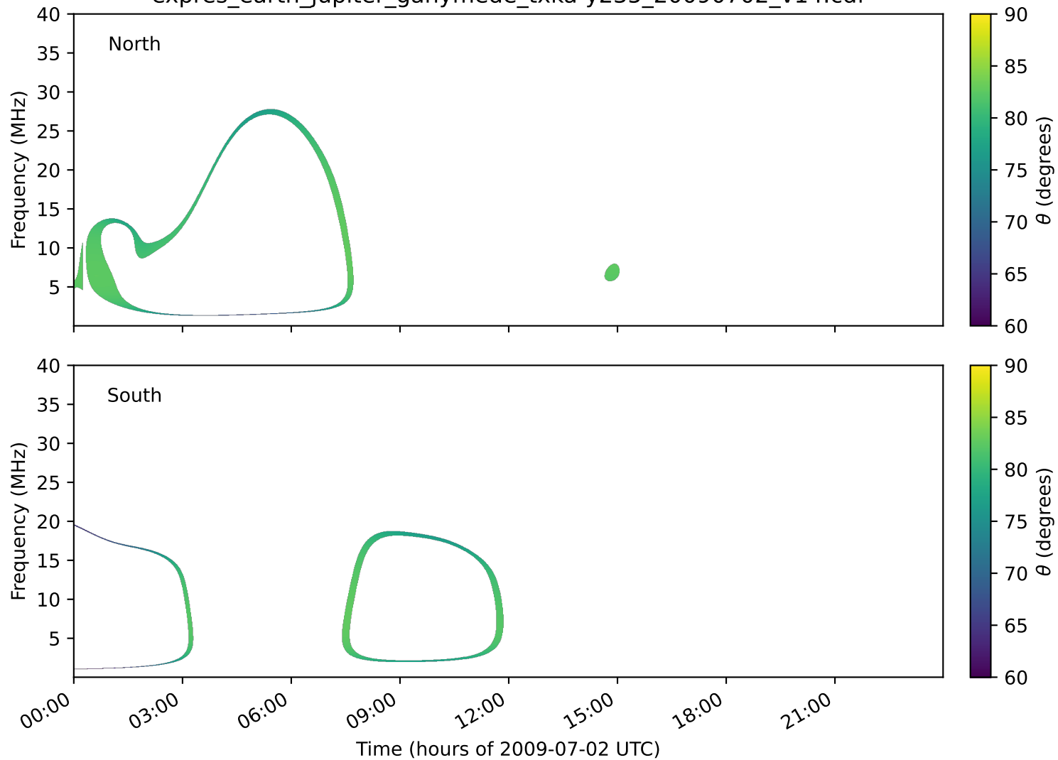
expres_earth_jupiter_ganymede_txka-y235_20090702_v14.cdf
