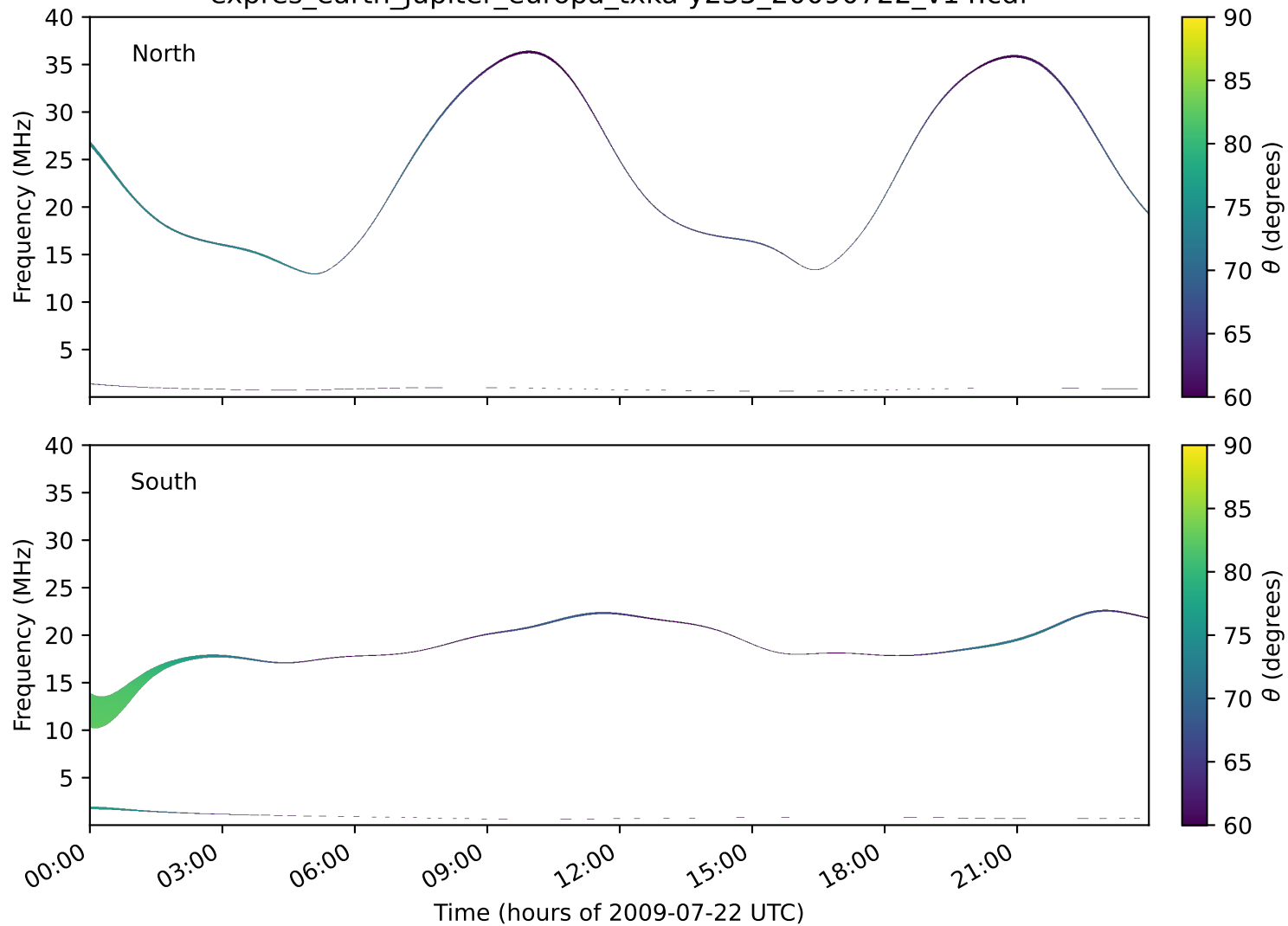
expres_earth_jupiter_europa_txka-y235_20090722_v14.cdf
