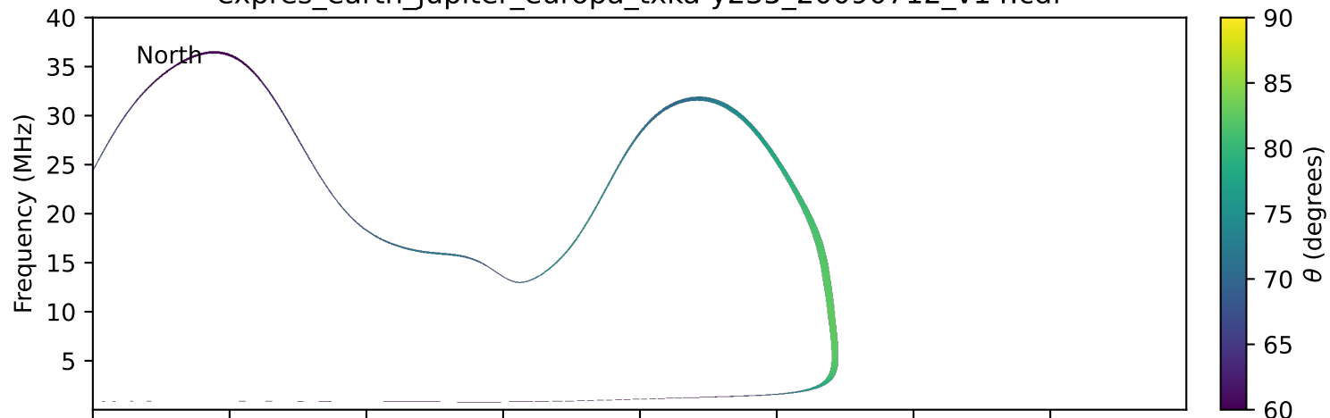
expres_earth_jupiter_europa_txka-y235_20090712_v14.cdf
