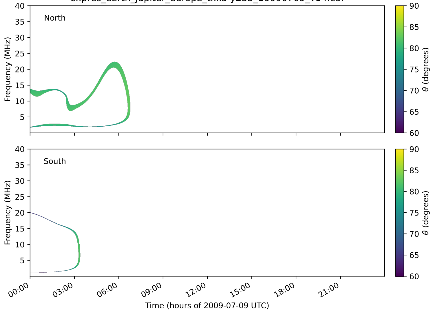
expres_earth_jupiter_europa_txka-y235_20090709_v14.cdf
