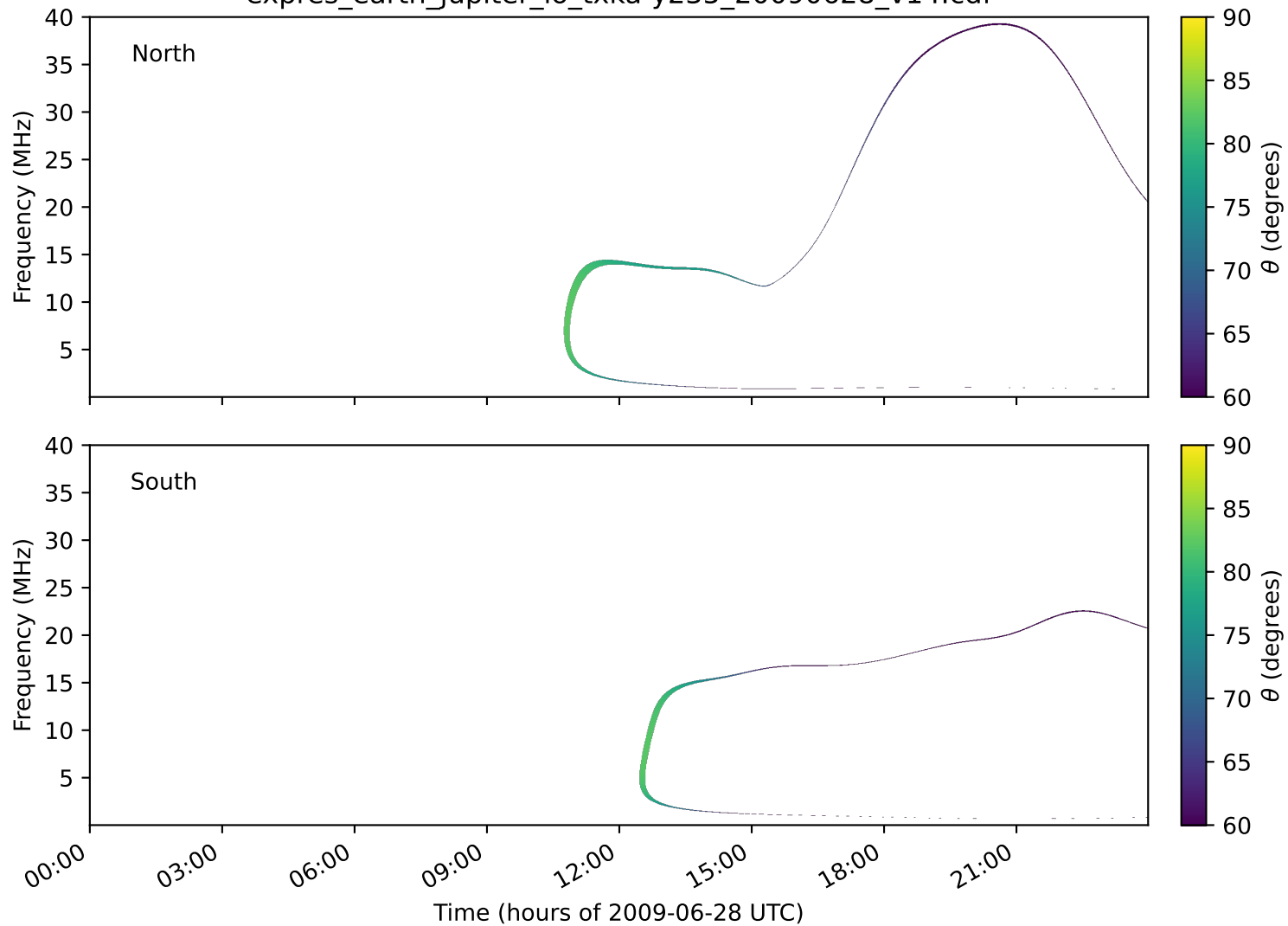
expres_earth_jupiter_io_txka-y235_20090628_v14.cdf
