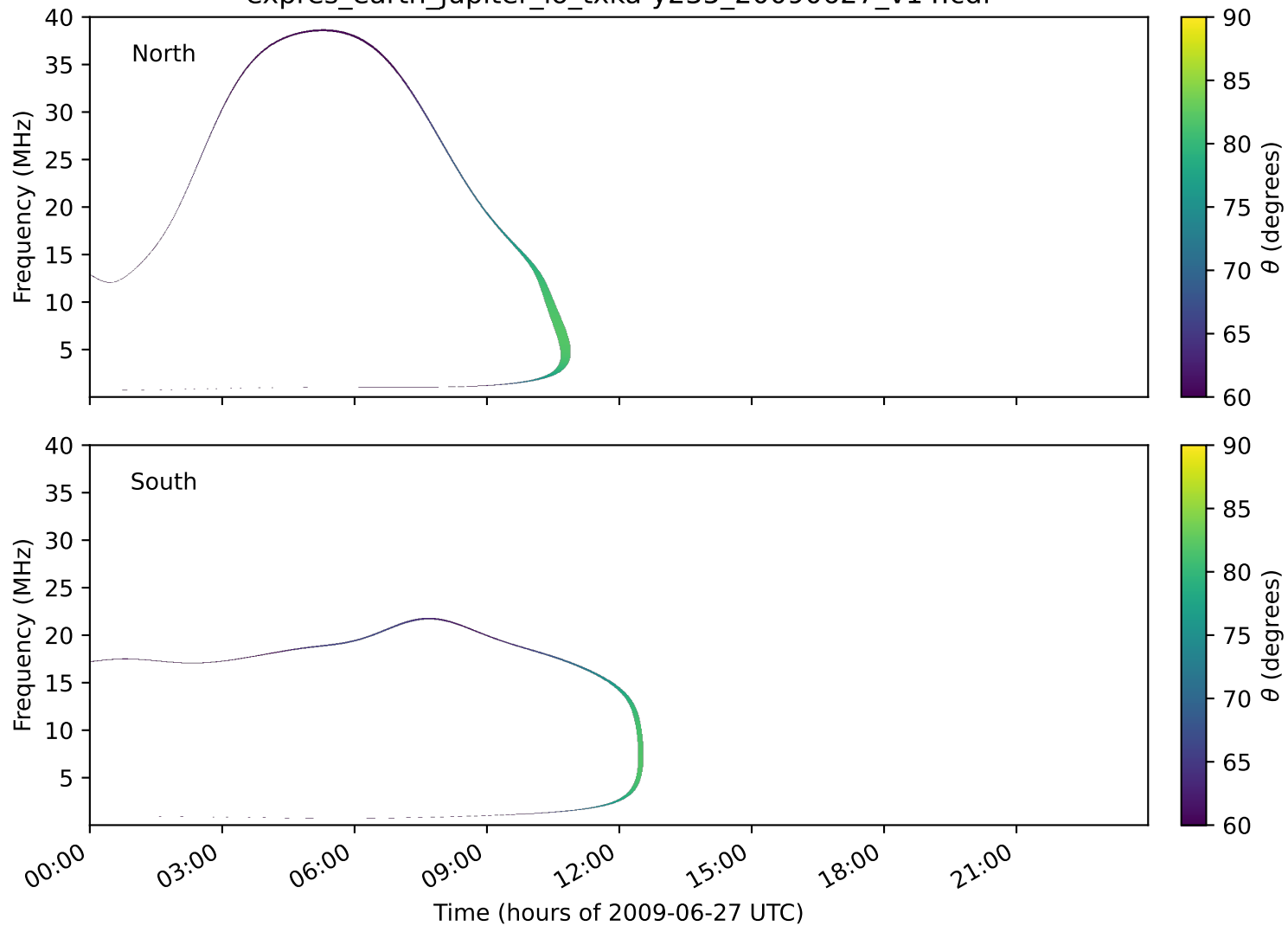
expres_earth_jupiter_io_txka-y235_20090627_v14.cdf
