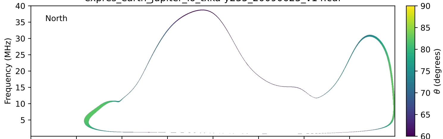
expres_earth_jupiter_io_txka-y235_20090623_v14.cdf
