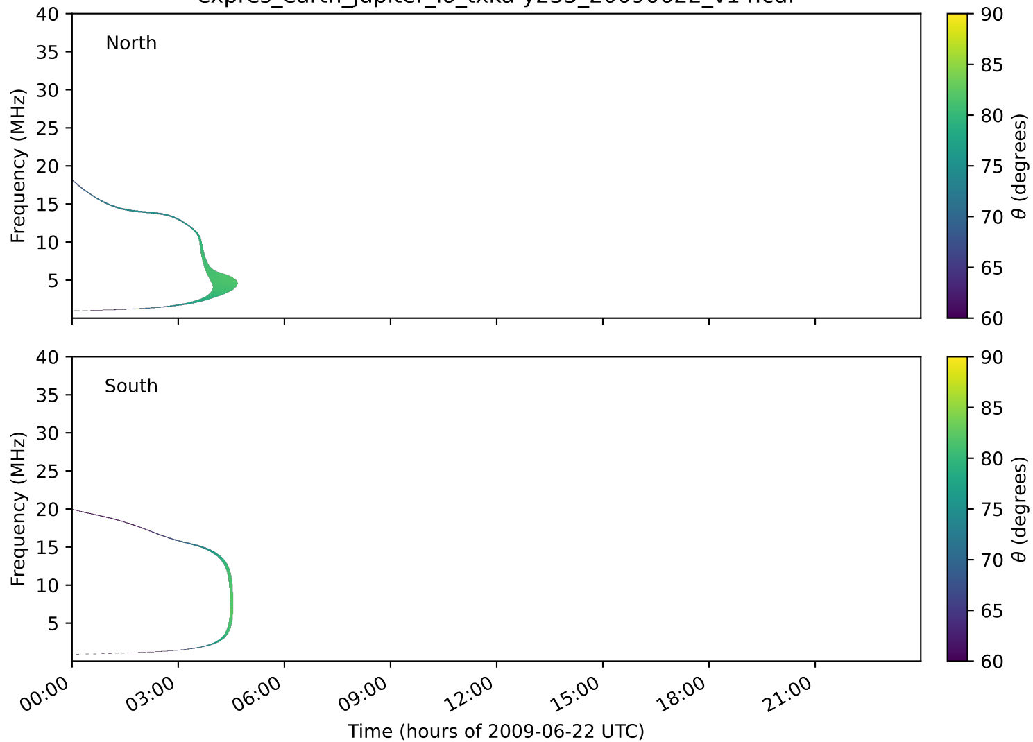
expres_earth_jupiter_io_txka-y235_20090622_v14.cdf
