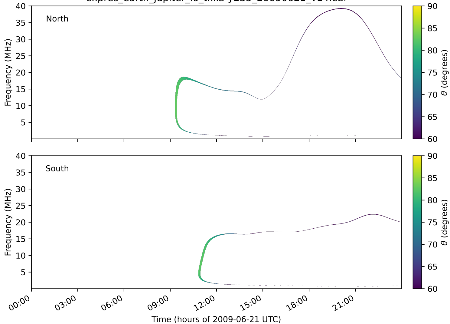
expres_earth_jupiter_io_txka-y235_20090621_v14.cdf
