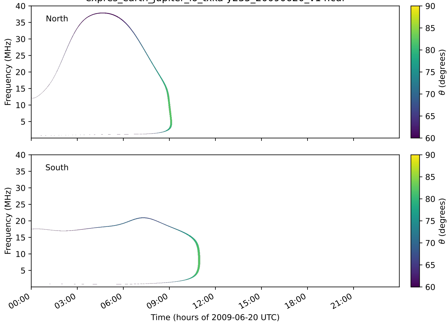
expres_earth_jupiter_io_txka-y235_20090620_v14.cdf
