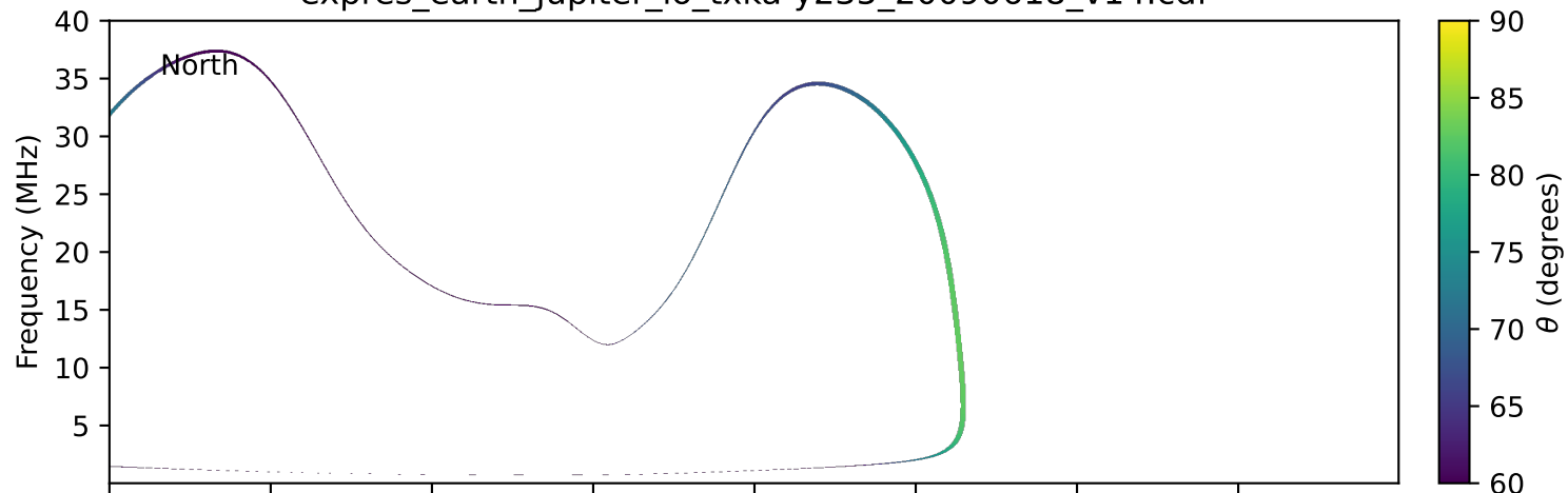
expres_earth_jupiter_io_txka-y235_20090618_v14.cdf
