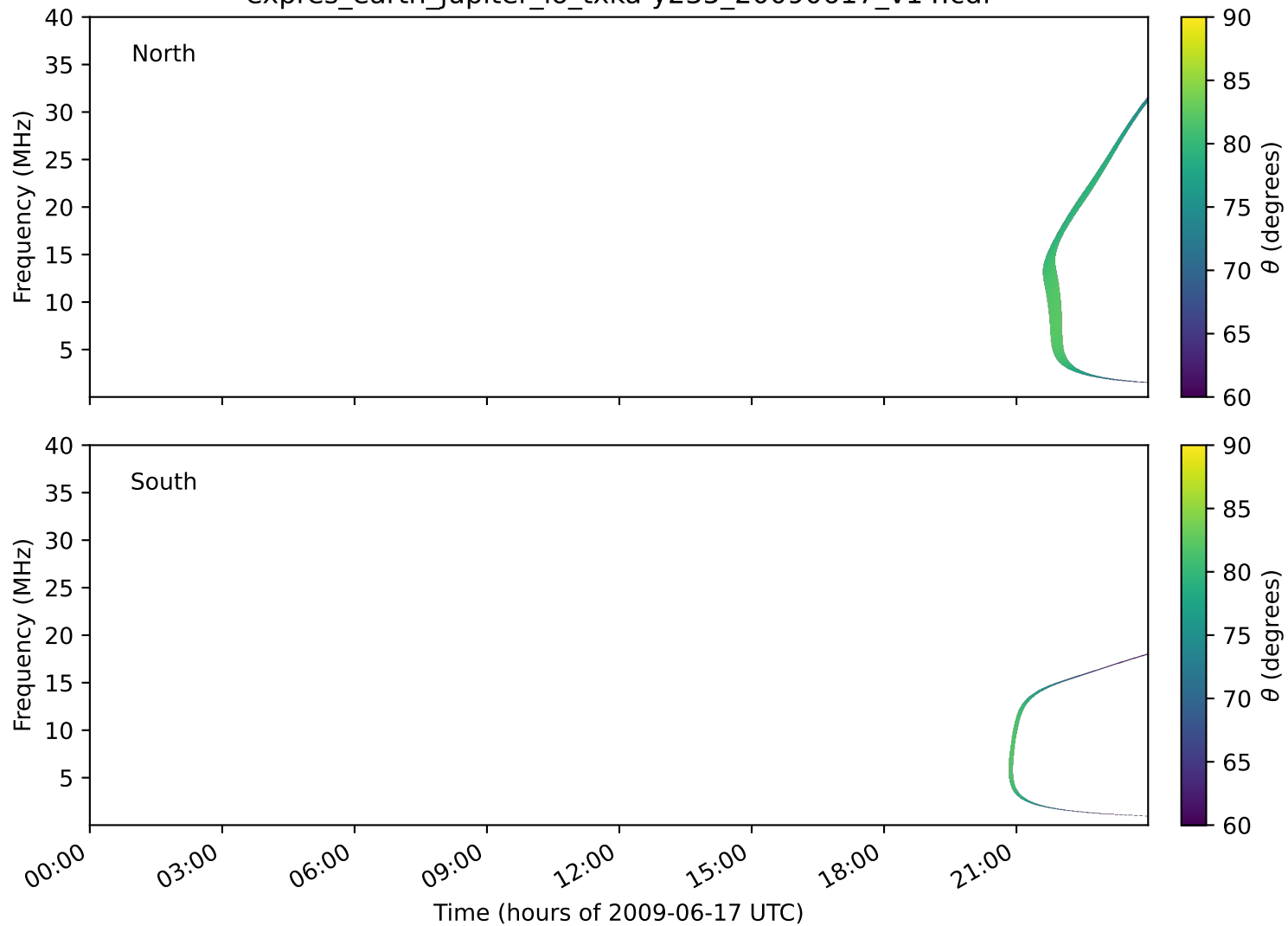
expres_earth_jupiter_io_txka-y235_20090617_v14.cdf
