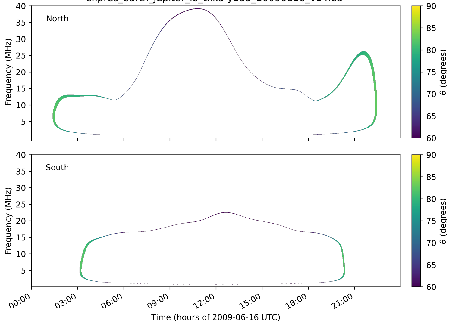
expres_earth_jupiter_io_txka-y235_20090616_v14.cdf
