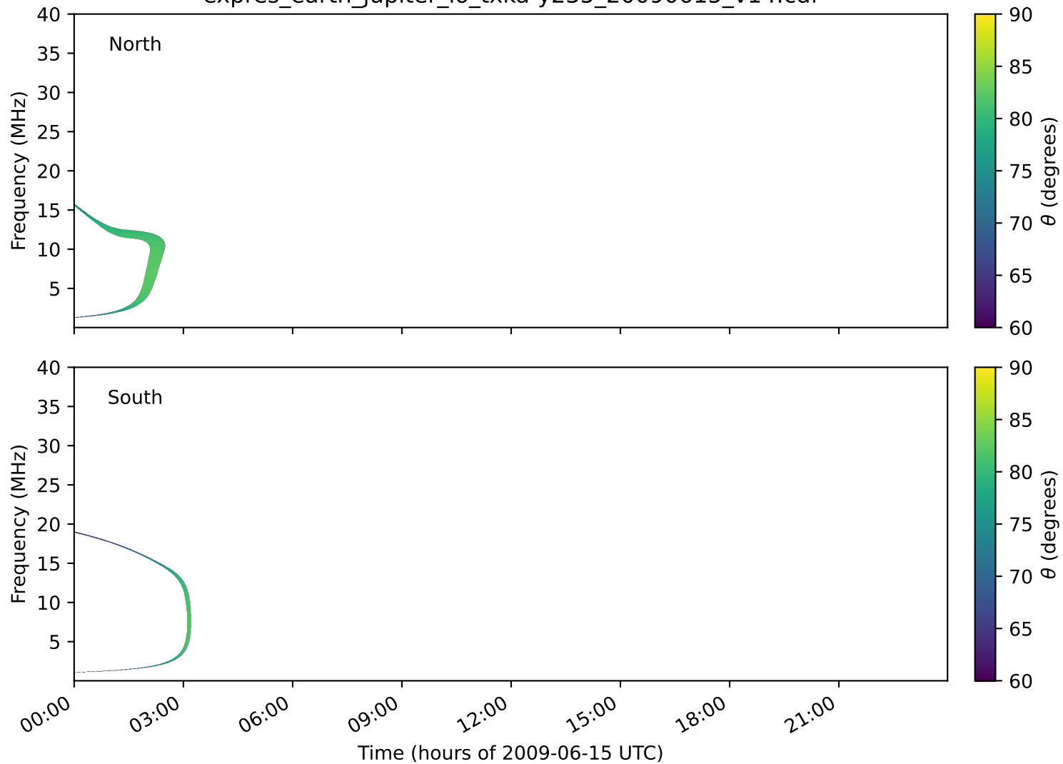
expres_earth_jupiter_io_txka-y235_20090615_v14.cdf
