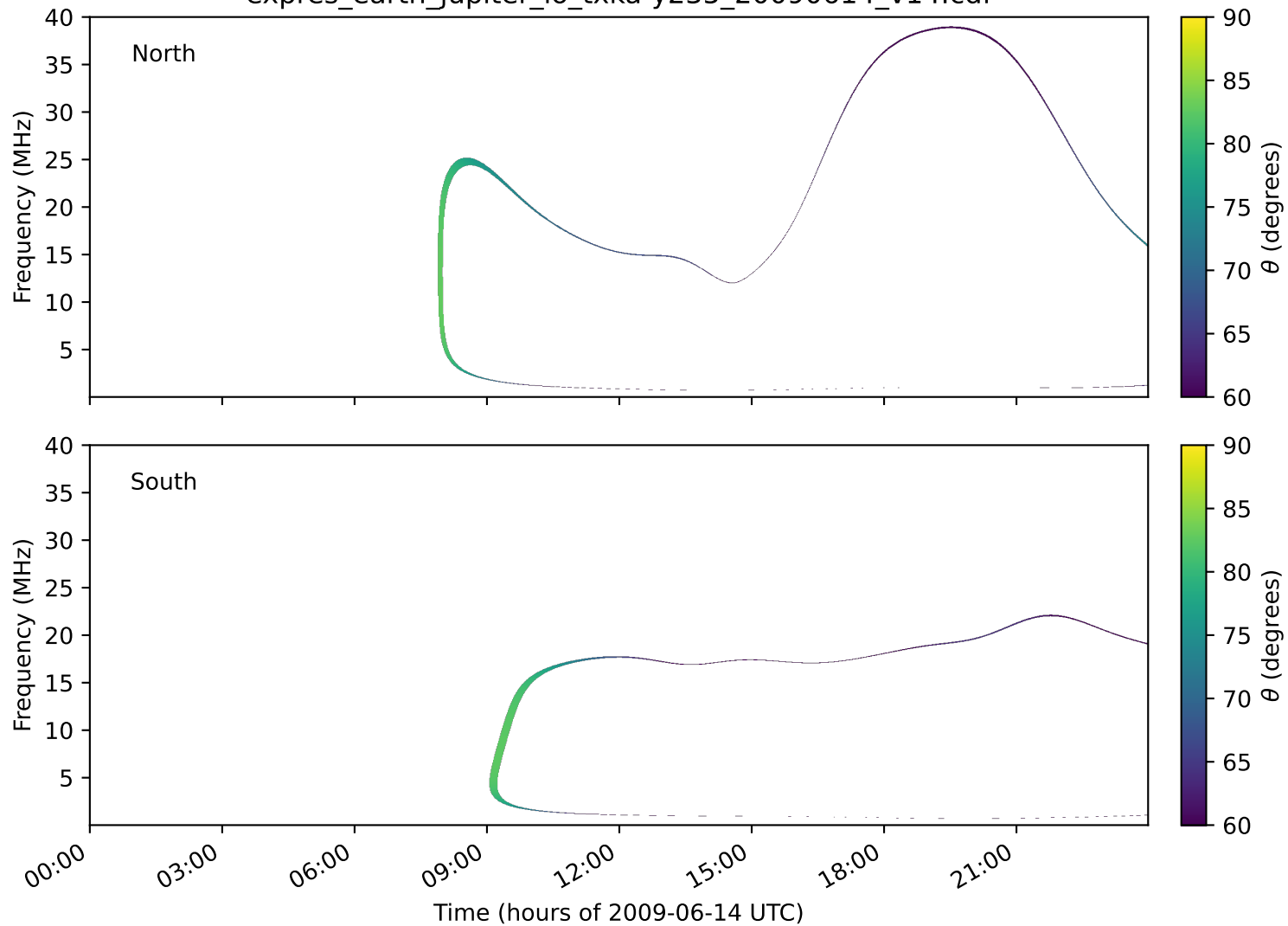
expres_earth_jupiter_io_txka-y235_20090614_v14.cdf
