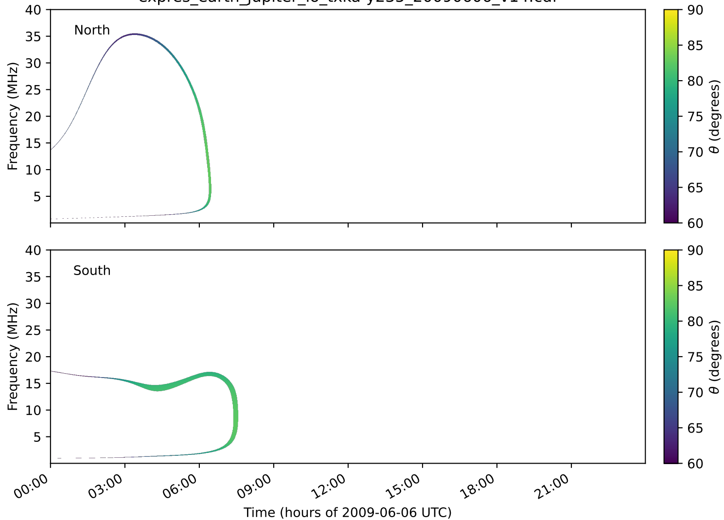
expres_earth_jupiter_io_txka-y235_20090606_v14.cdf
