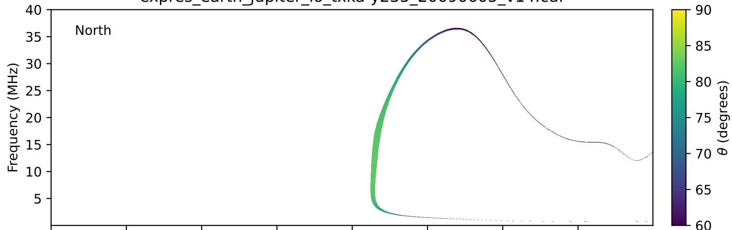
expres_earth_jupiter_io_txka-y235_20090605_v14.cdf
