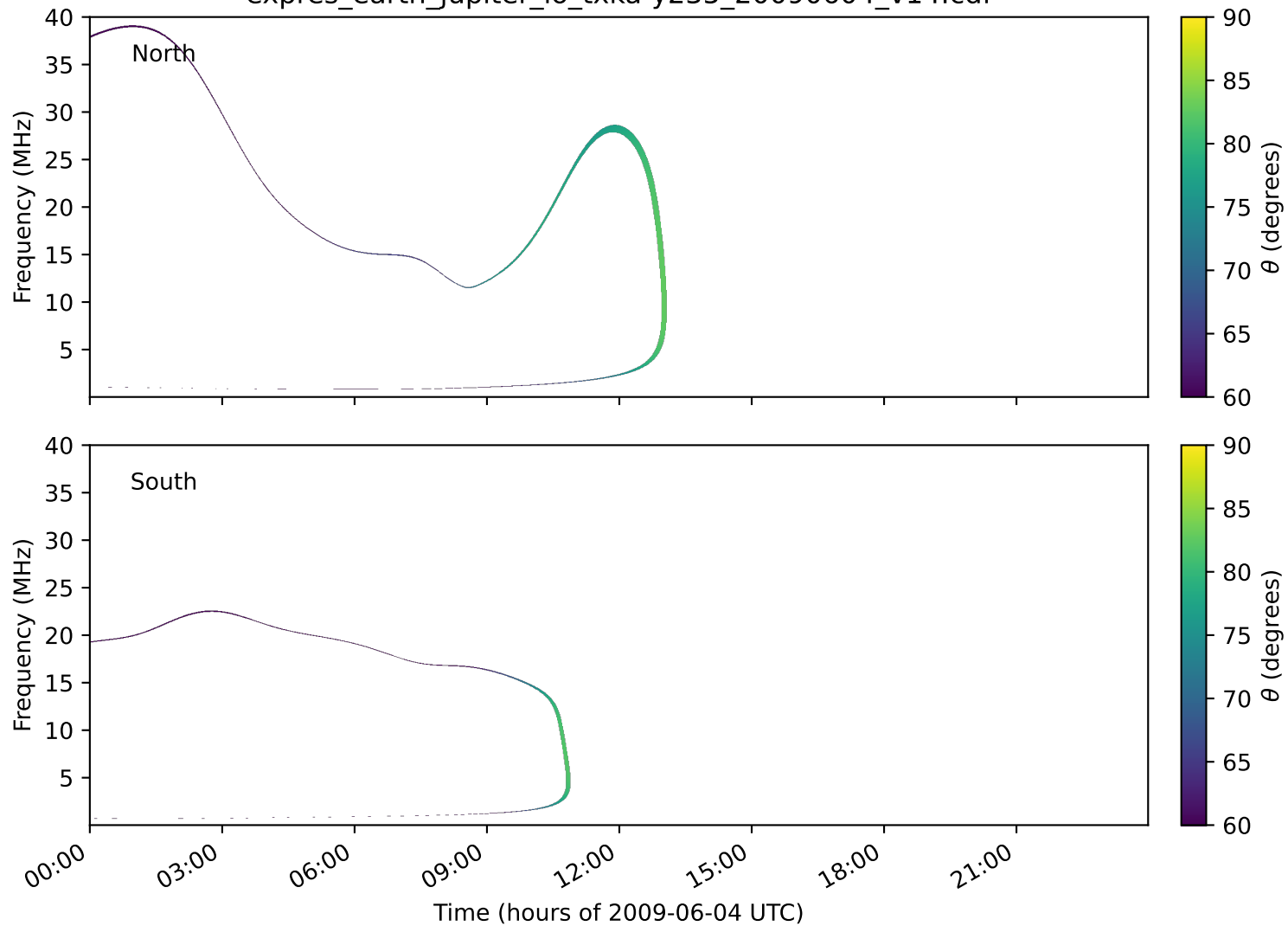
expres_earth_jupiter_io_txka-y235_20090604_v14.cdf
