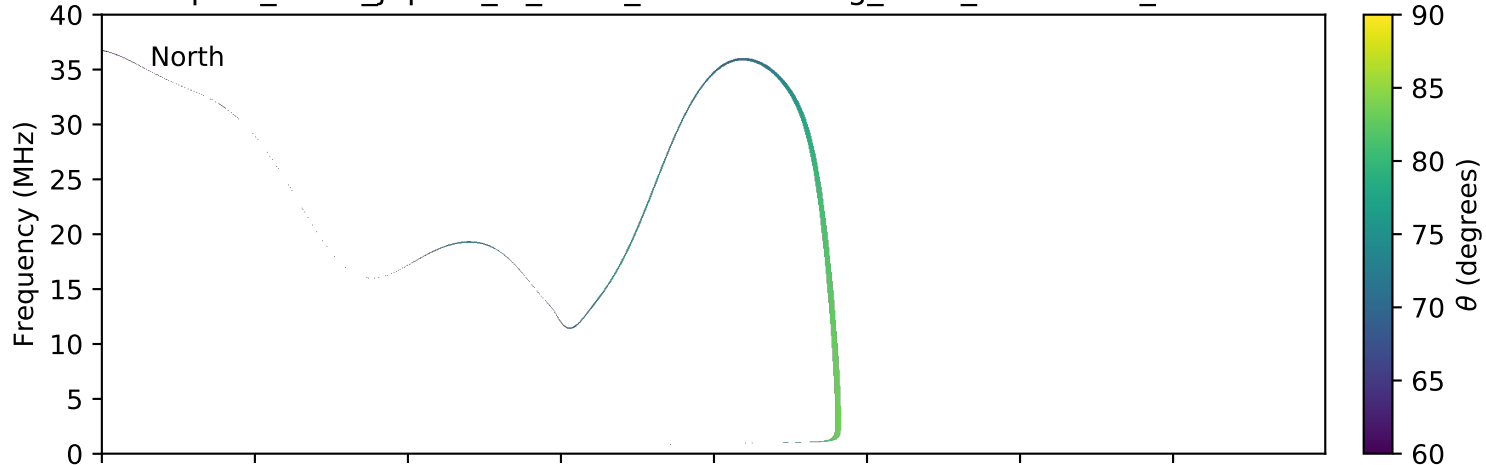
expres_earth_jupiter_io_isaac_lossc-wid1deg_3kev_20090611_v01.cdf
