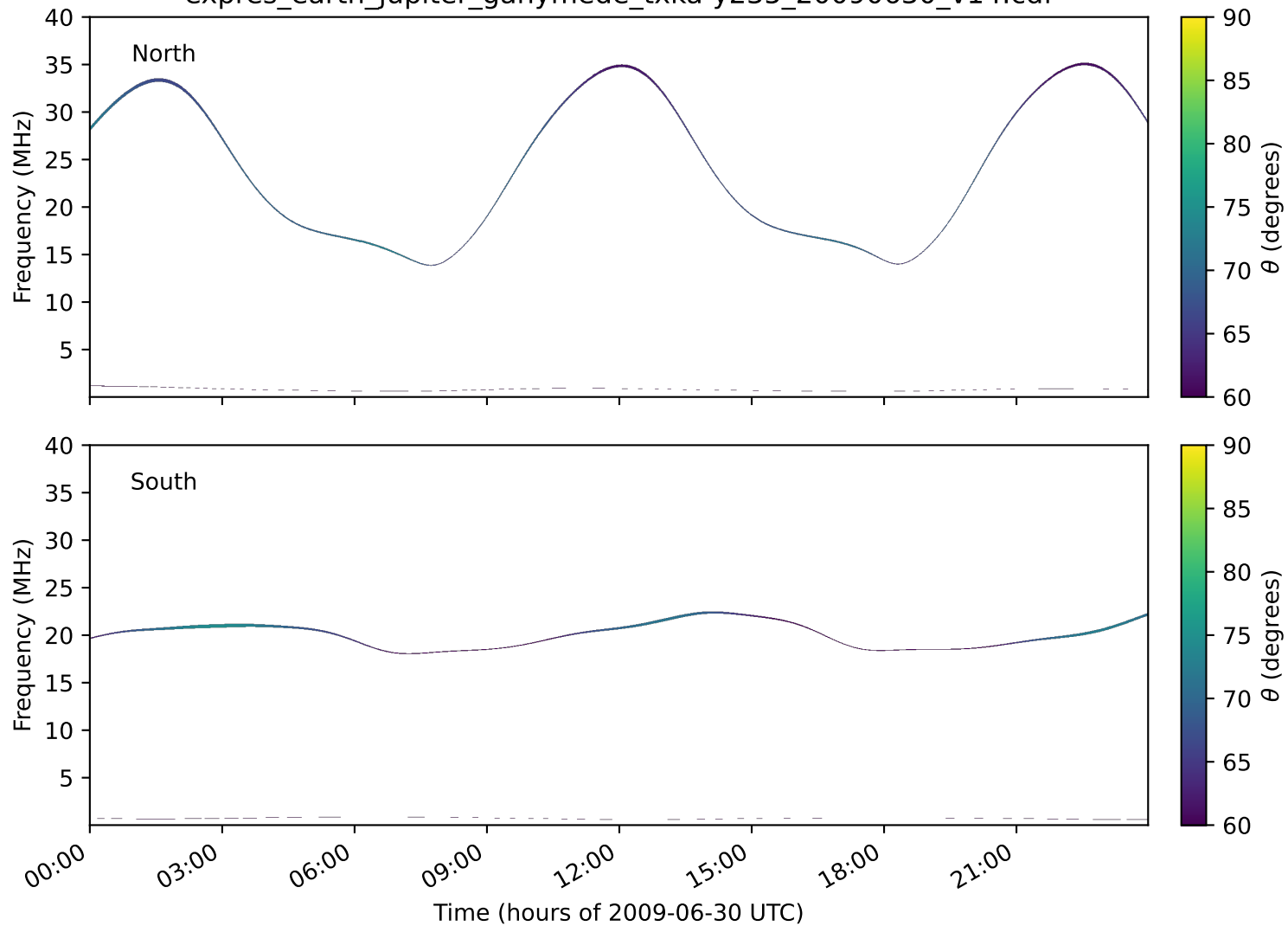
expres_earth_jupiter_ganymede_txka-y235_20090630_v14.cdf
