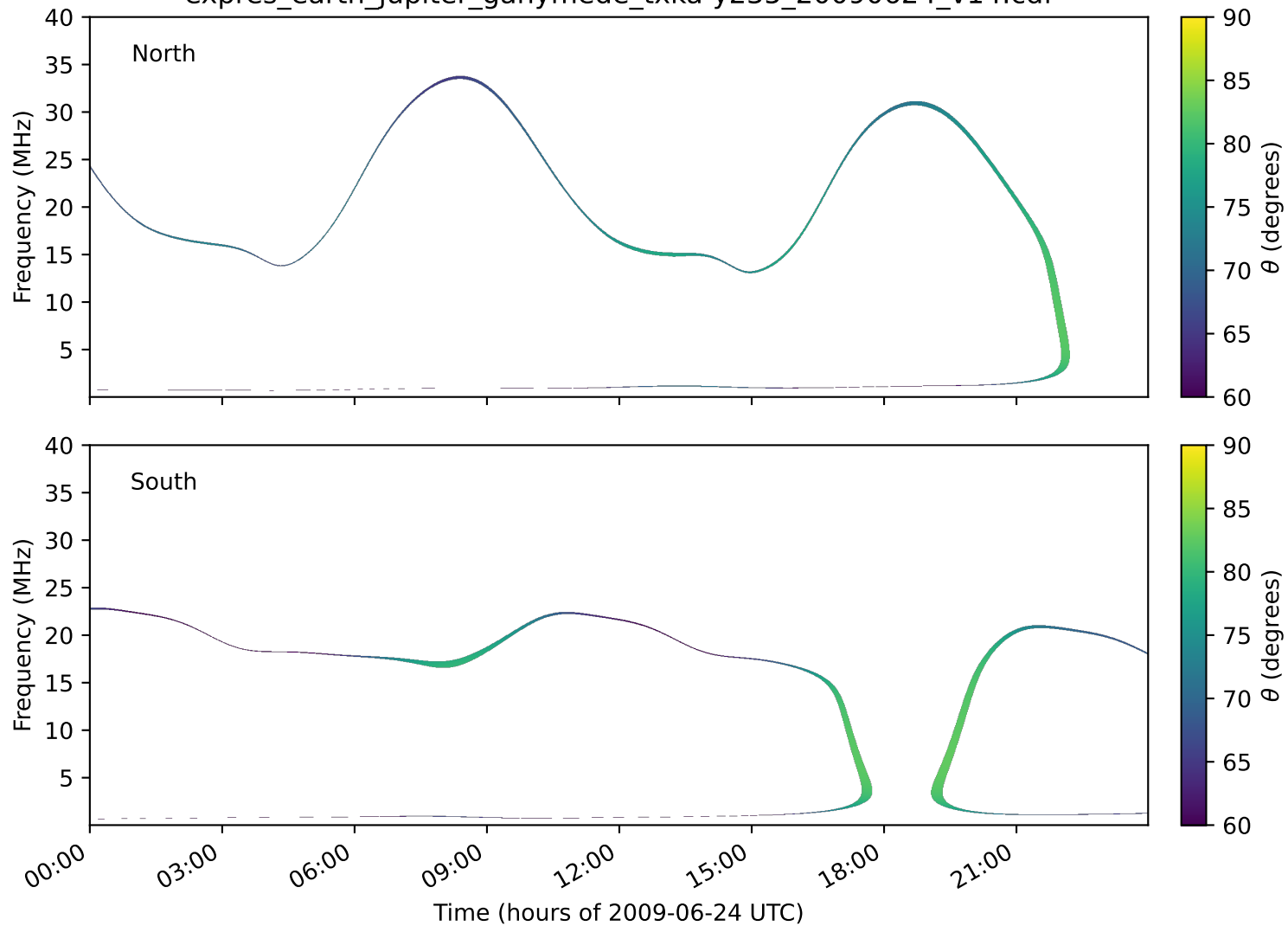
expres_earth_jupiter_ganymede_txka-y235_20090624_v14.cdf
