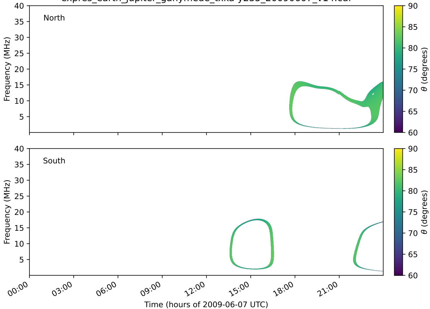
expres_earth_jupiter_ganymede_txka-y235_20090607_v14.cdf
