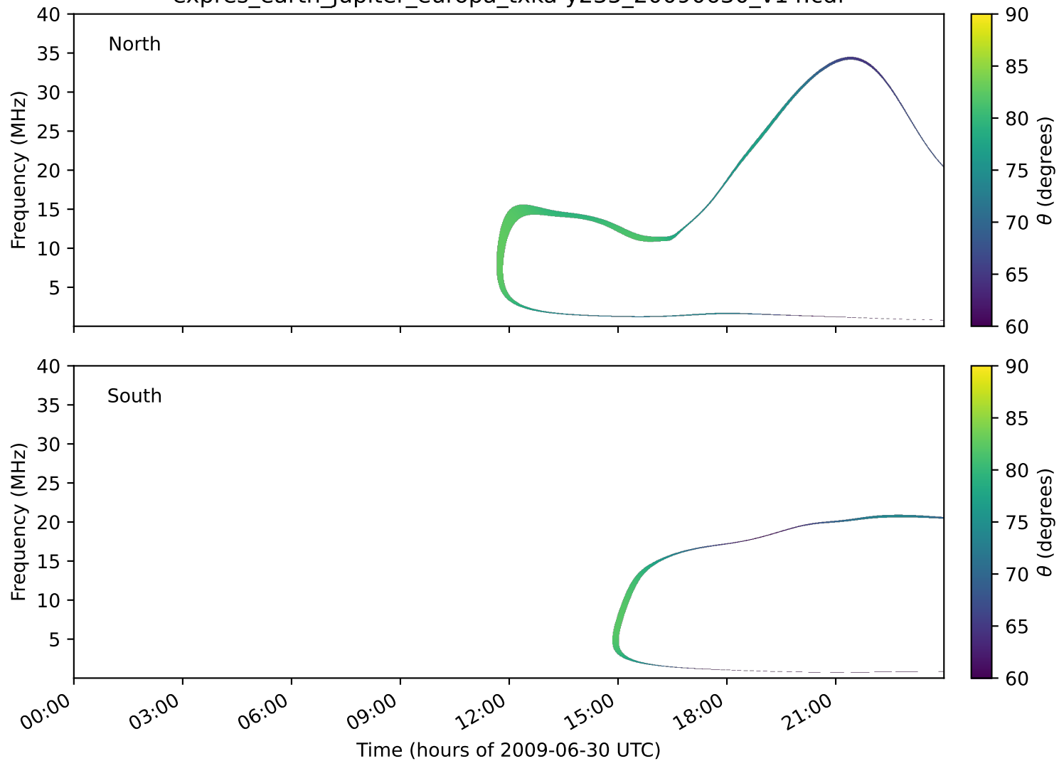
expres_earth_jupiter_europa_txka-y235_20090630_v14.cdf
