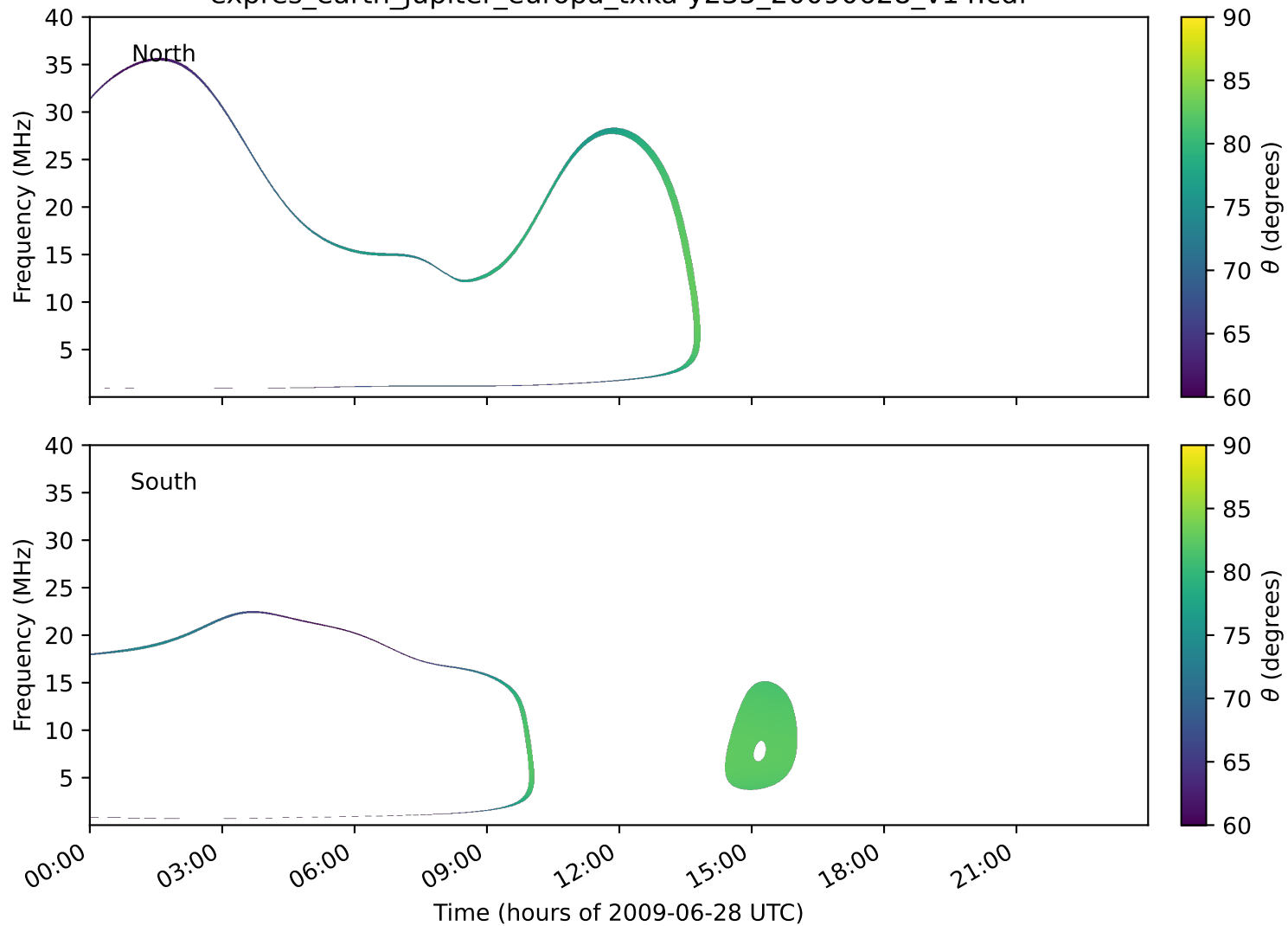
expres_earth_jupiter_europa_txka-y235_20090628_v14.cdf
