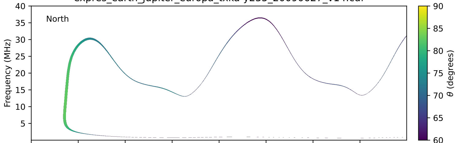
expres_earth_jupiter_europa_txka-y235_20090627_v14.cdf
