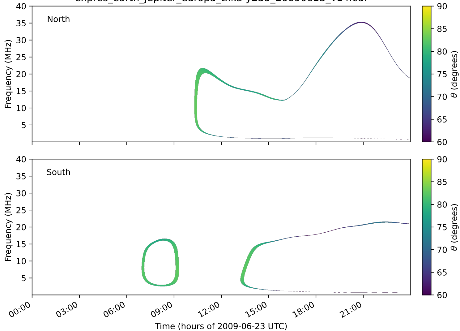
expres_earth_jupiter_europa_txka-y235_20090623_v14.cdf
