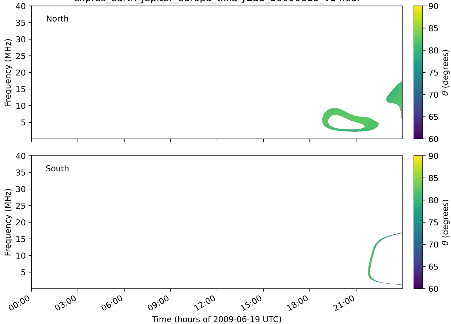
expres_earth_jupiter_europa_txka-y235_20090619_v14.cdf
