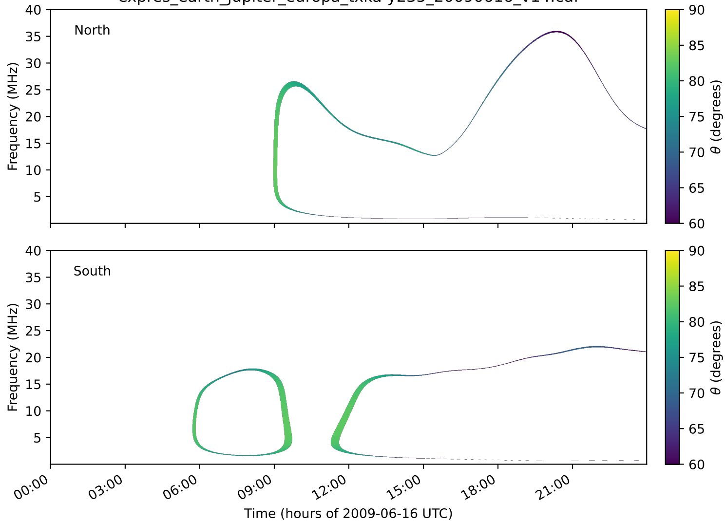
expres_earth_jupiter_europa_txka-y235_20090616_v14.cdf
