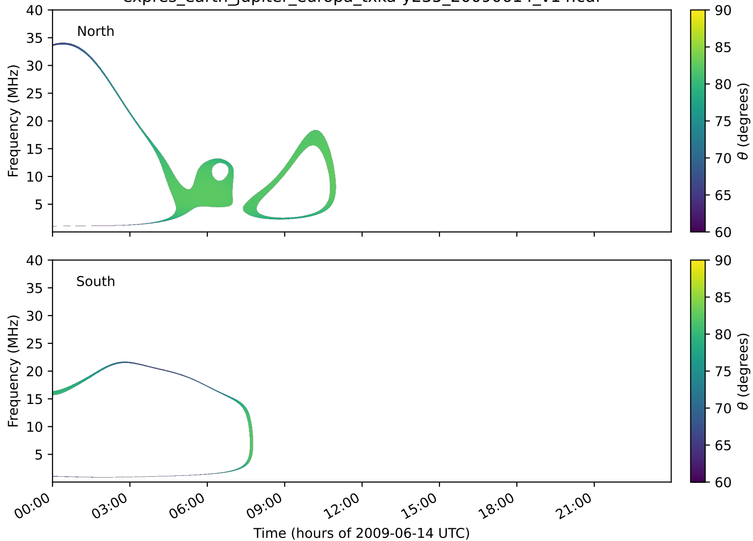
expres_earth_jupiter_europa_txka-y235_20090614_v14.cdf
