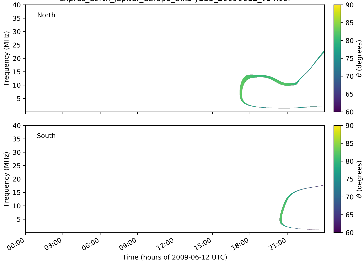
expres_earth_jupiter_europa_txka-y235_20090612_v14.cdf
