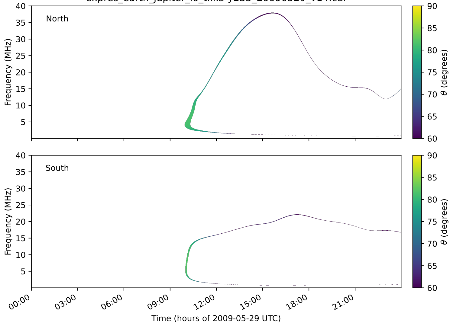
expres_earth_jupiter_io_txka-y235_20090529_v14.cdf
