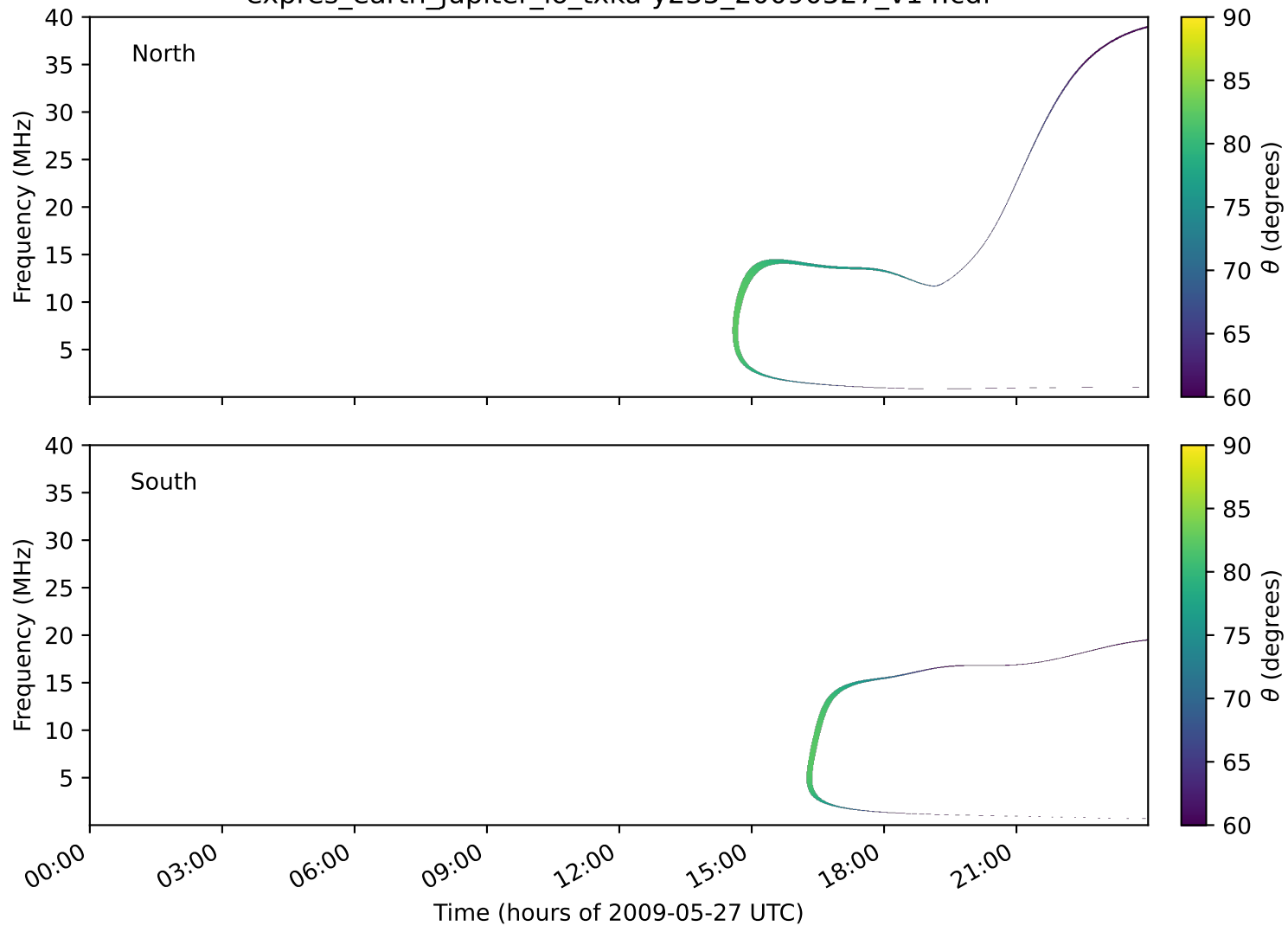
expres_earth_jupiter_io_txka-y235_20090527_v14.cdf
