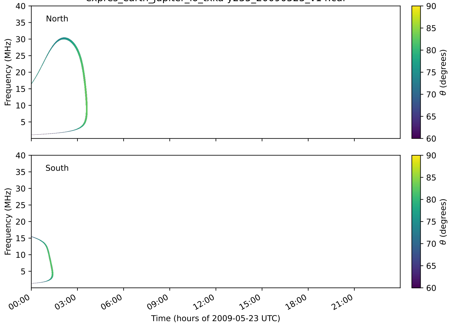
expres_earth_jupiter_io_txka-y235_20090523_v14.cdf
