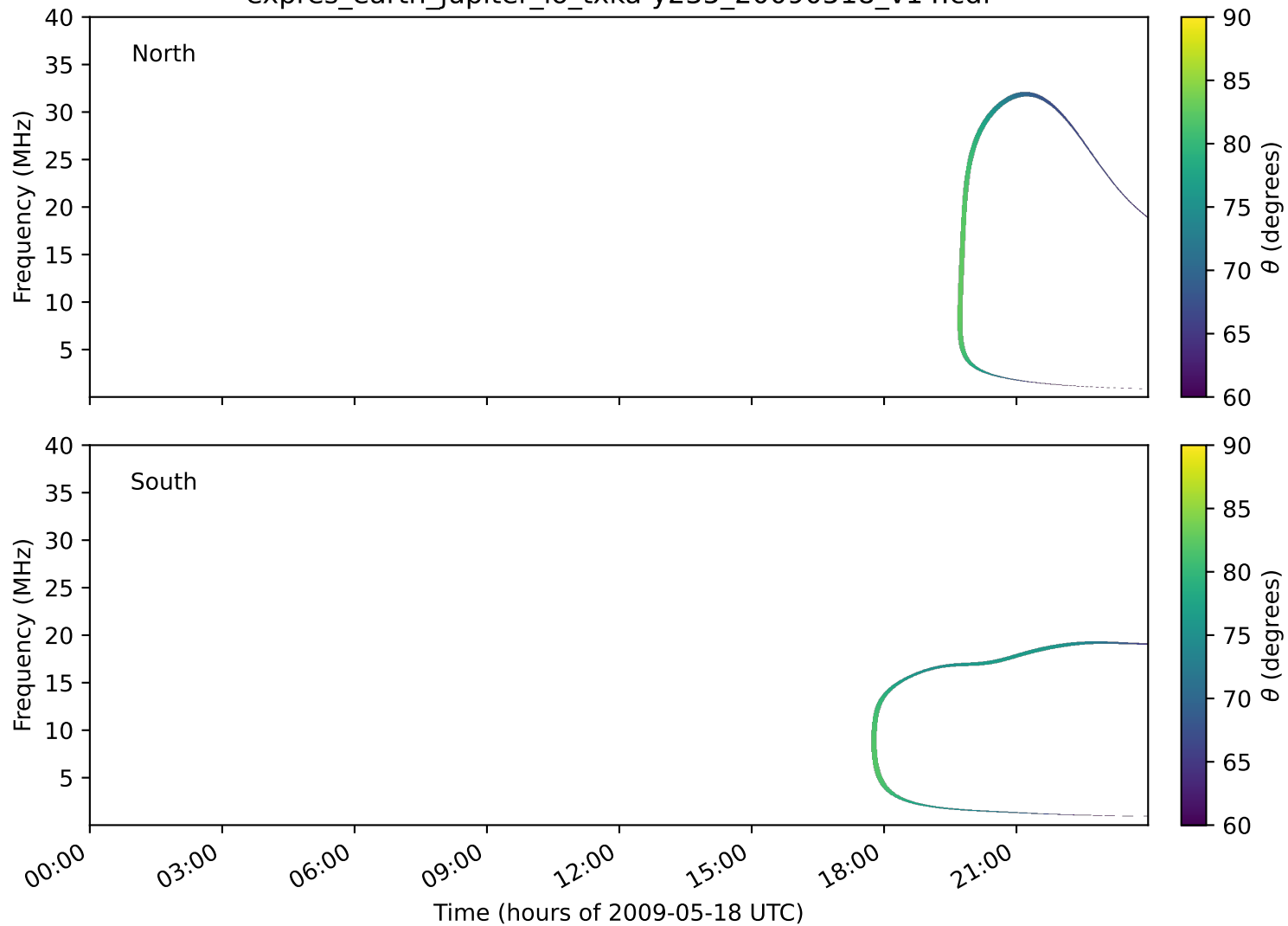
expres_earth_jupiter_io_txka-y235_20090518_v14.cdf
