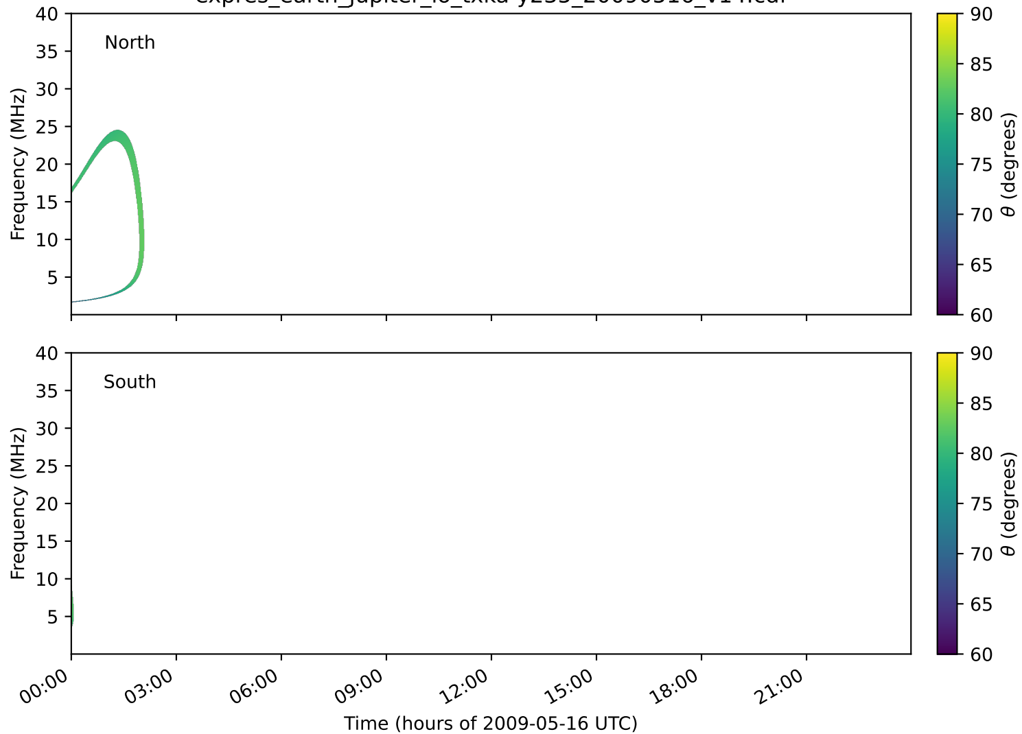
expres_earth_jupiter_io_txka-y235_20090516_v14.cdf
