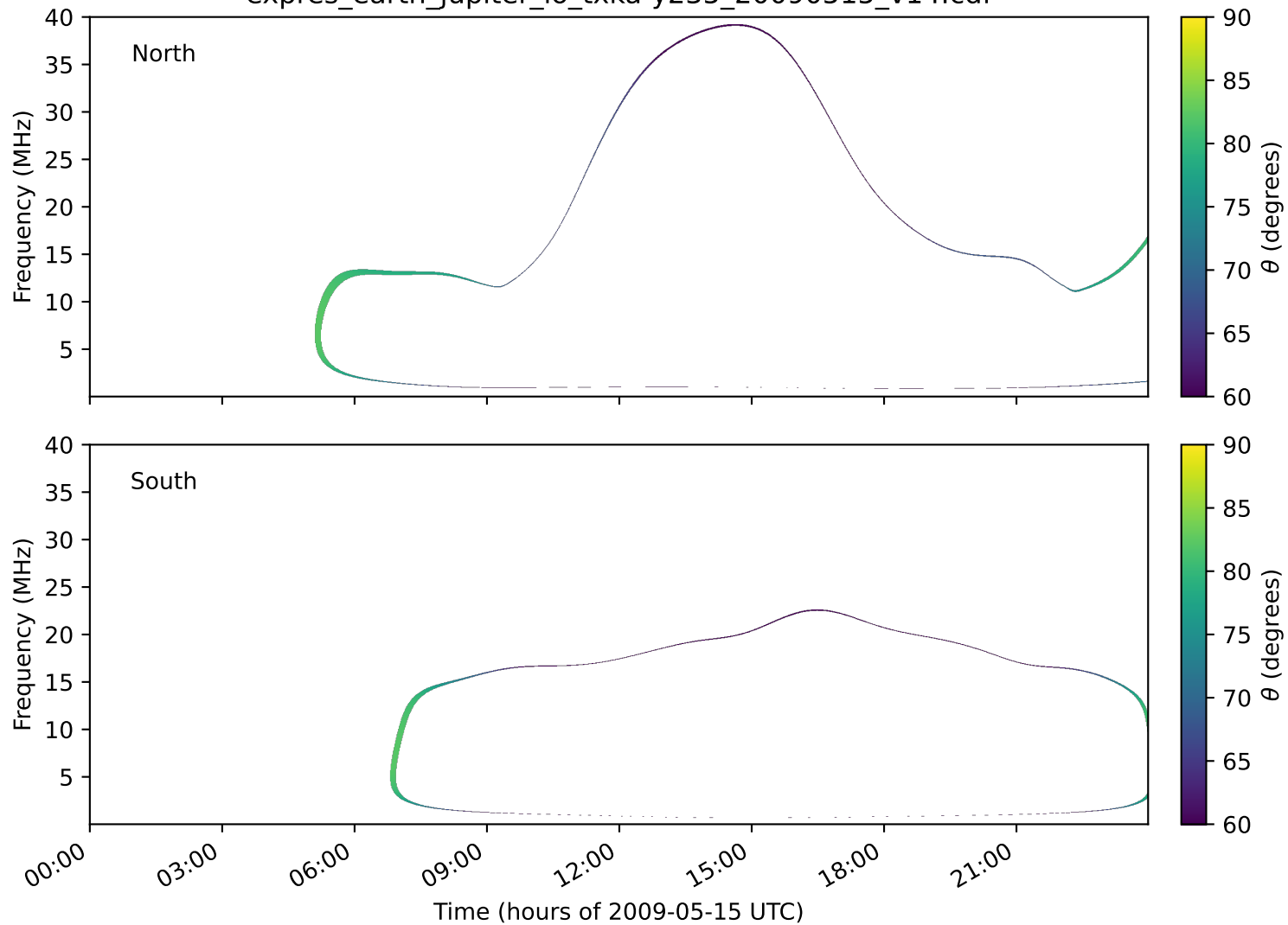
expres_earth_jupiter_io_txka-y235_20090515_v14.cdf
