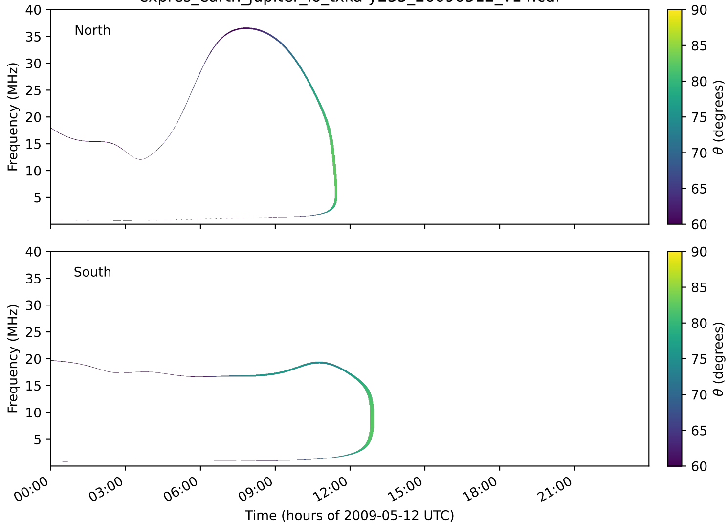
expres_earth_jupiter_io_txka-y235_20090512_v14.cdf
