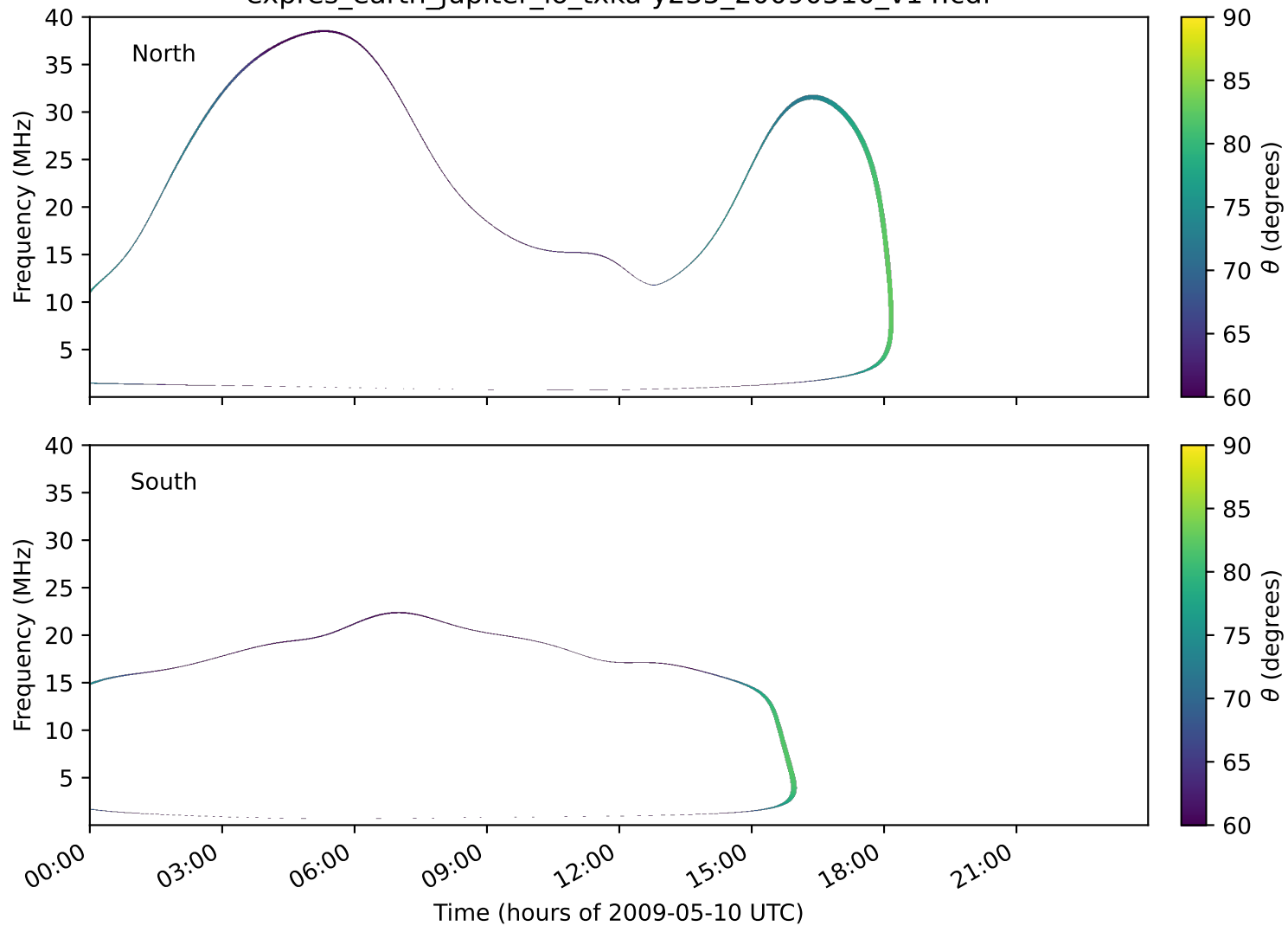
expres_earth_jupiter_io_txka-y235_20090510_v14.cdf
