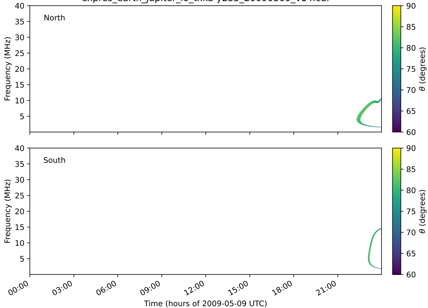
expres_earth_jupiter_io_txka-y235_20090509_v14.cdf
