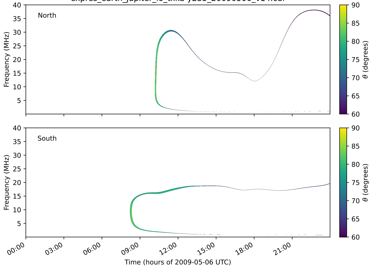
expres_earth_jupiter_io_txka-y235_20090506_v14.cdf
