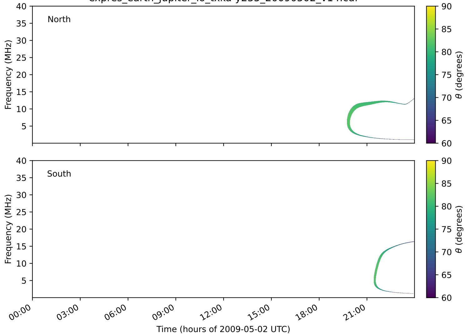
expres_earth_jupiter_io_txka-y235_20090502_v14.cdf
