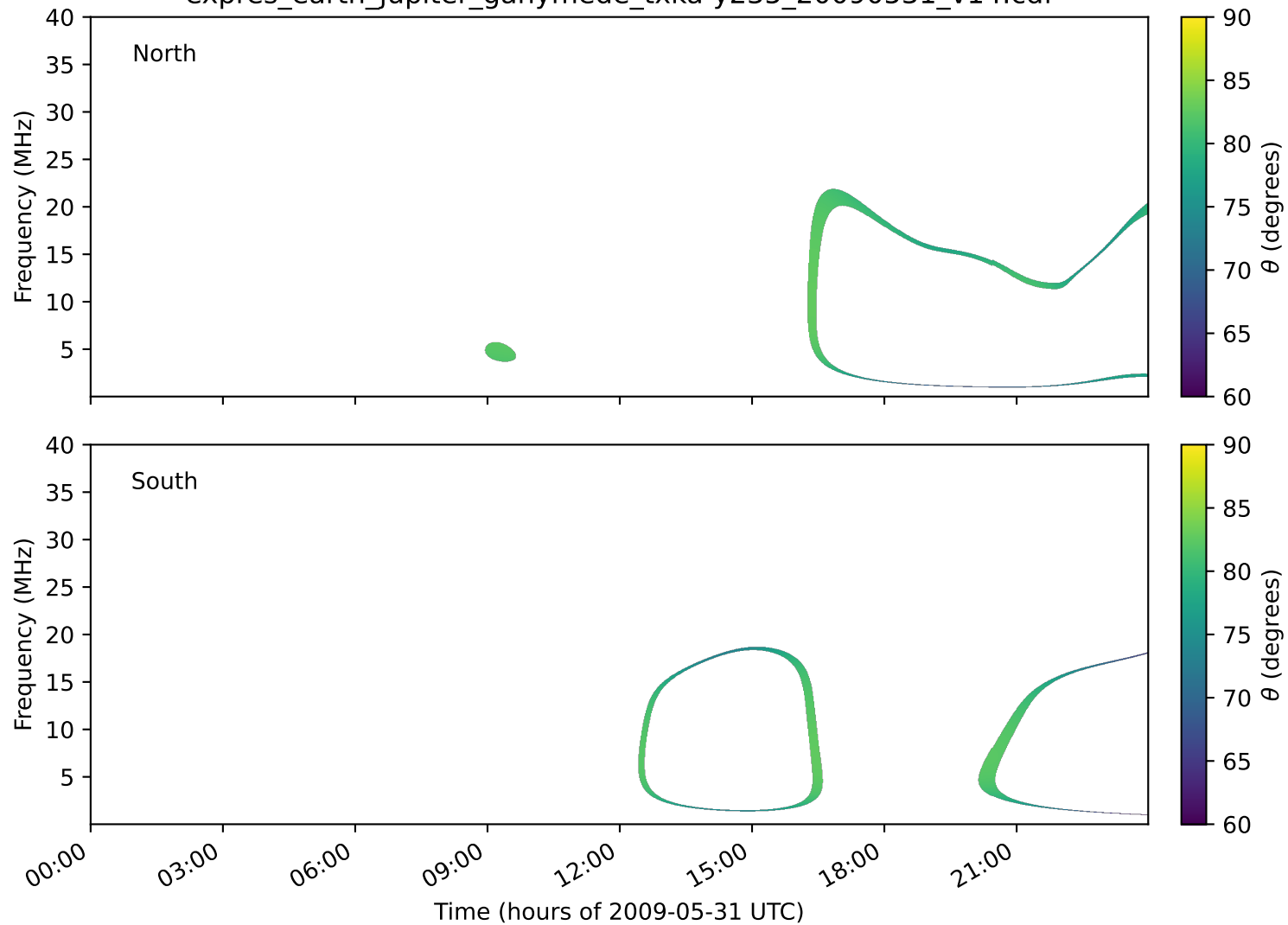
expres_earth_jupiter_ganymede_txka-y235_20090531_v14.cdf
