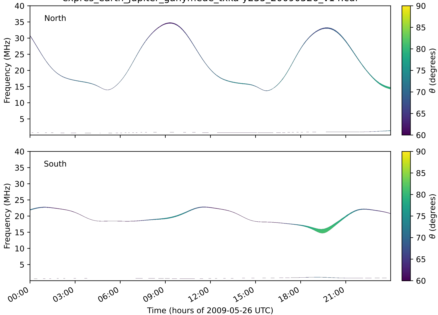
expres_earth_jupiter_ganymede_txka-y235_20090526_v14.cdf
