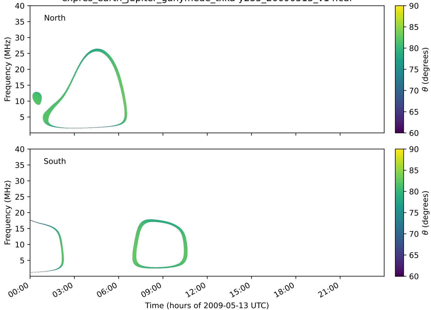
expres_earth_jupiter_ganymede_txka-y235_20090513_v14.cdf
