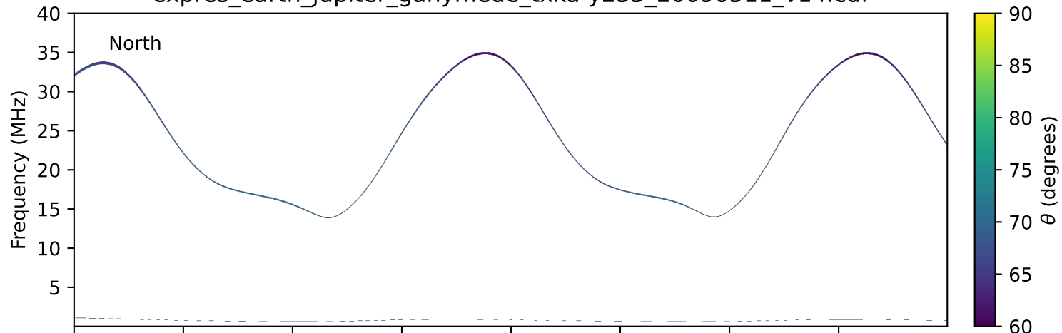
expres_earth_jupiter_ganymede_txka-y235_20090511_v14.cdf
