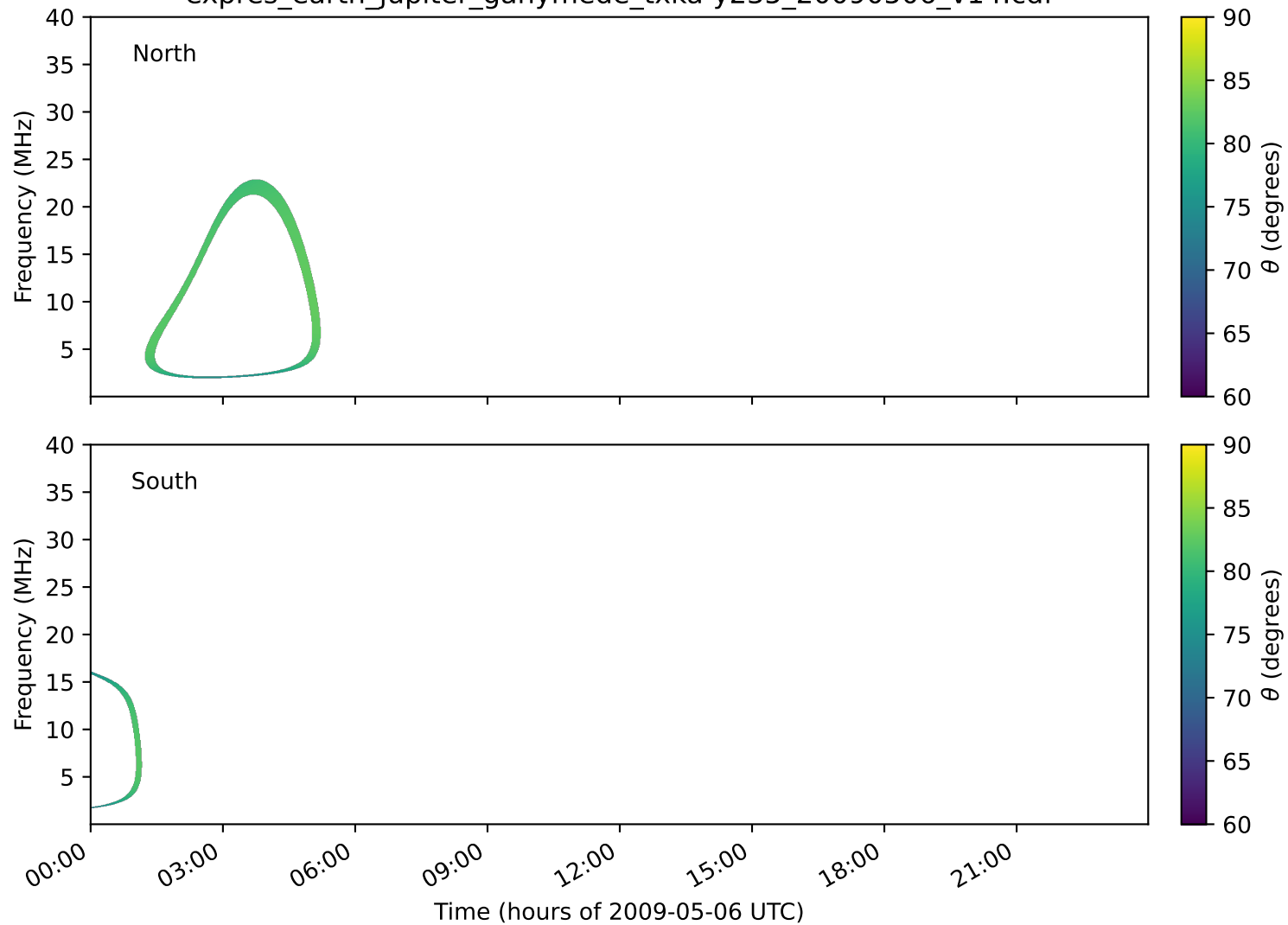
expres_earth_jupiter_ganymede_txka-y235_20090506_v14.cdf
