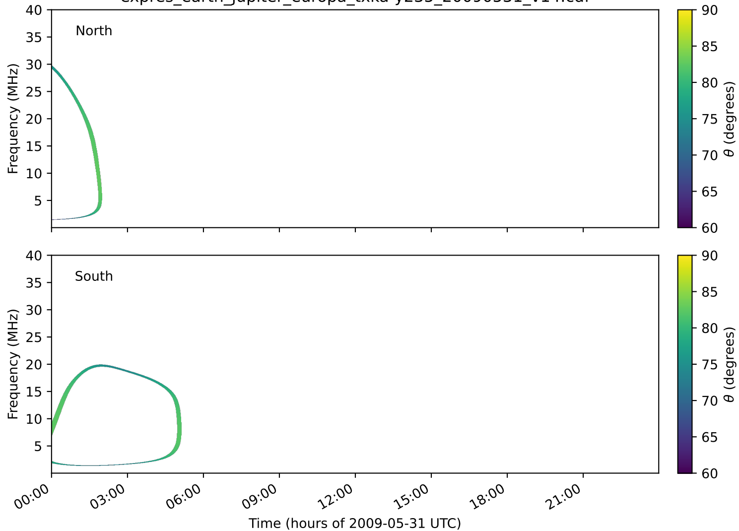
expres_earth_jupiter_europa_txka-y235_20090531_v14.cdf
