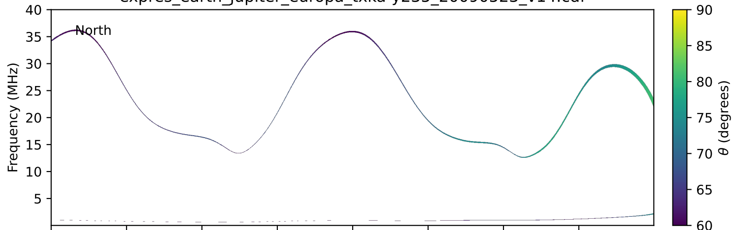
expres_earth_jupiter_europa_txka-y235_20090523_v14.cdf
